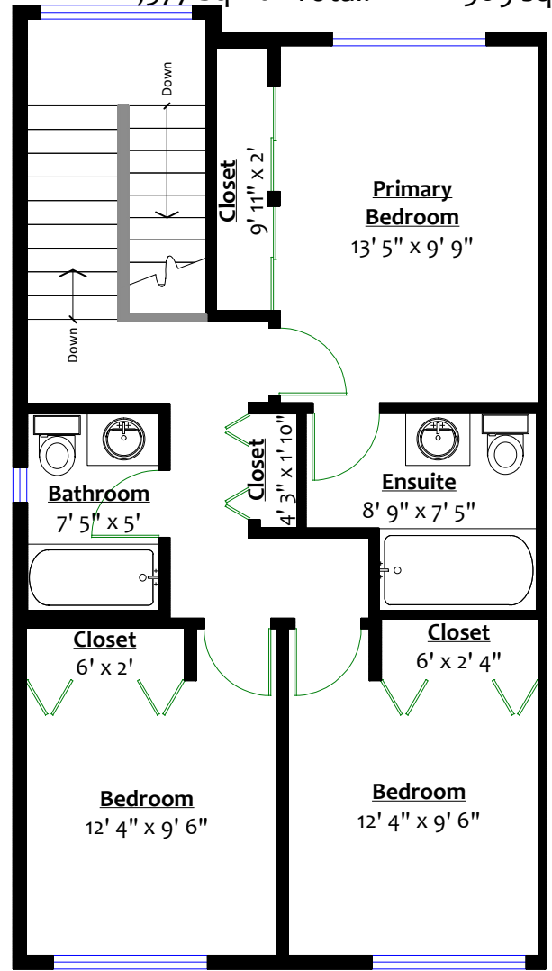
UPPER LEVEL Floor Area: 714 Sq. Ft. Ceiling Height: 8'
