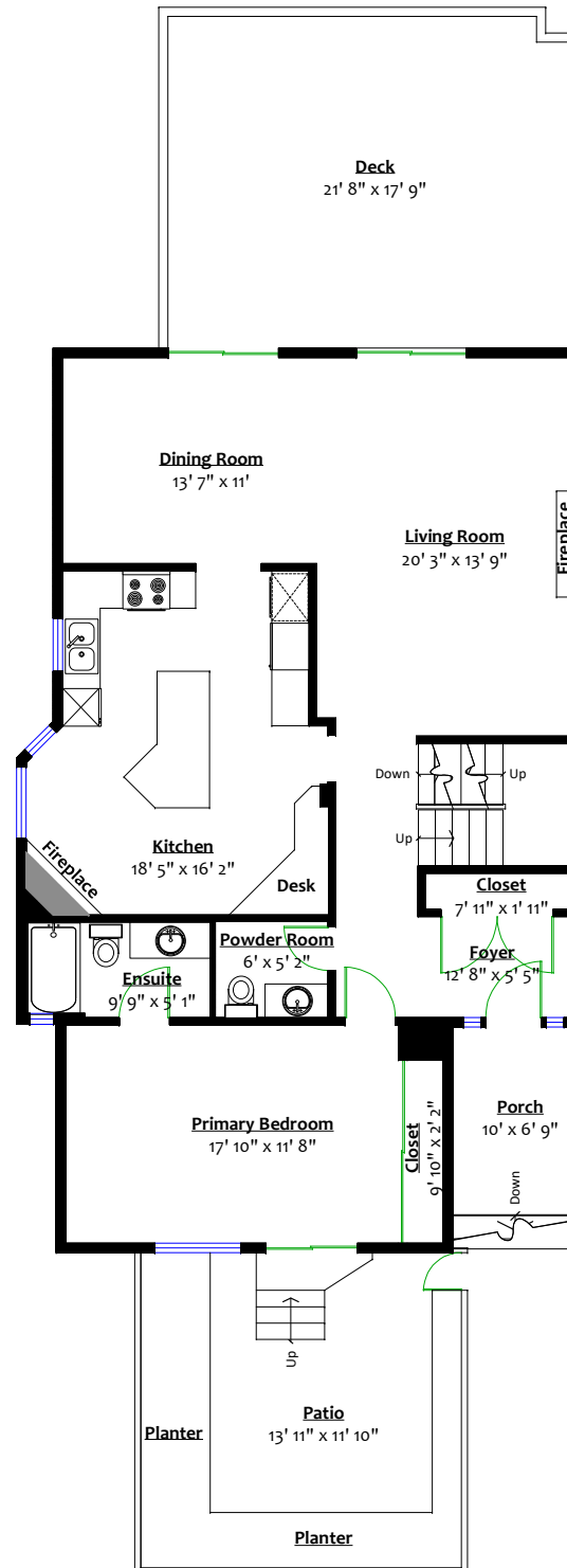
MAIN LEVEL Floor Area: 1,310 Sq. Ft. Ceiling Height: 8'
