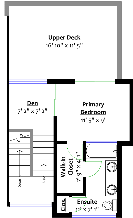
UPPER LEVEL Floor Area: 392 Sq. Ft. Ceiling Height: 8'
