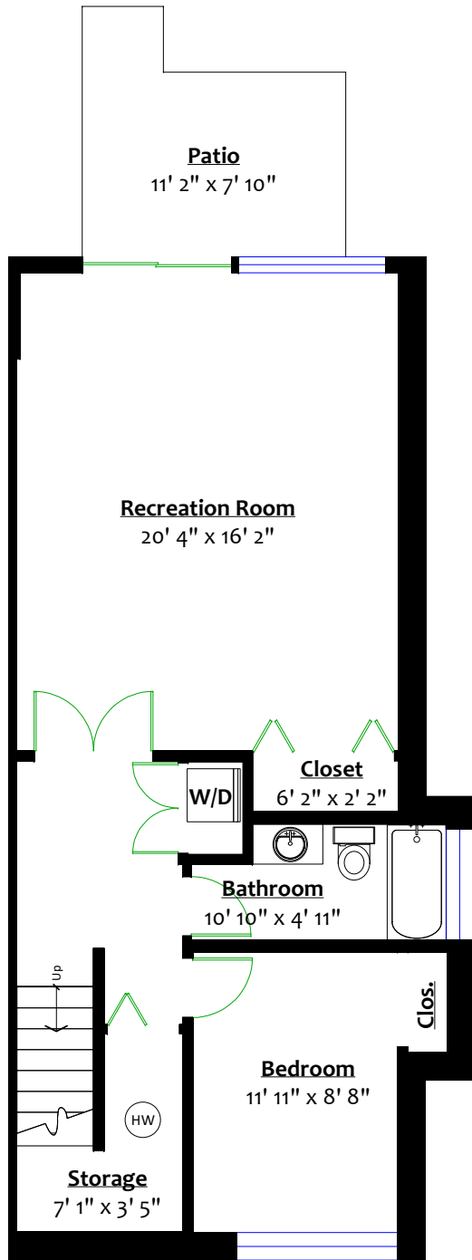
LOWER LEVEL Floor Area: 776 Sq. Ft. Ceiling Height: 8'
