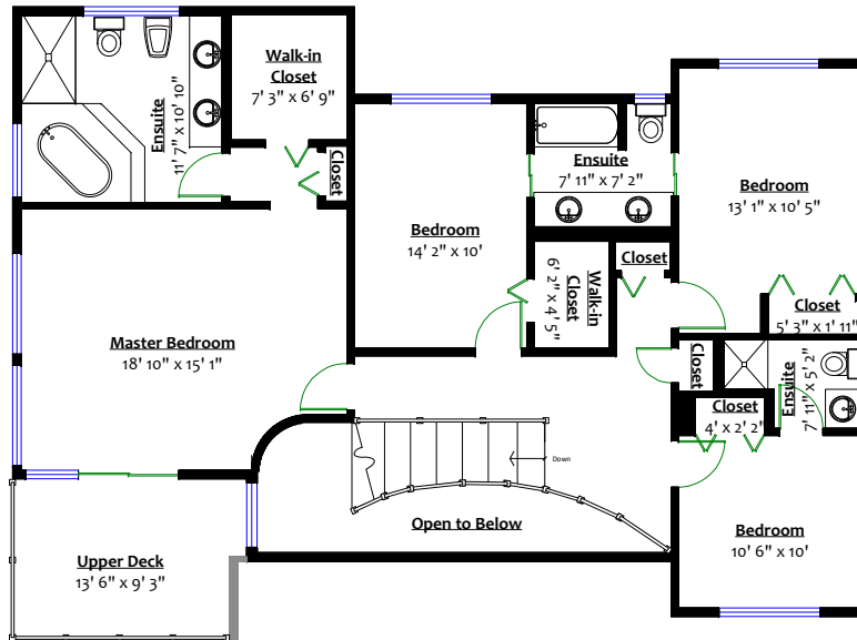
UPPER LEVEL Floor Area: 1,428 Sq. Ft. Ceiling Height: 7' 11"
